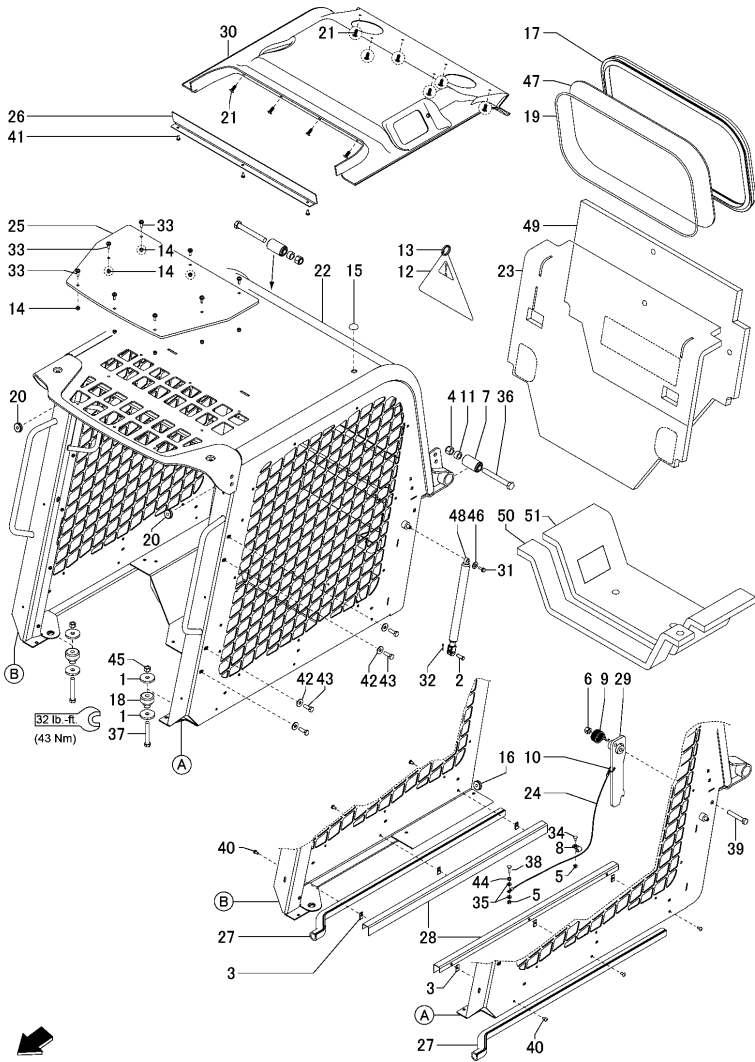
Fig.8. ROPS/FOPS ASSEMBLY
