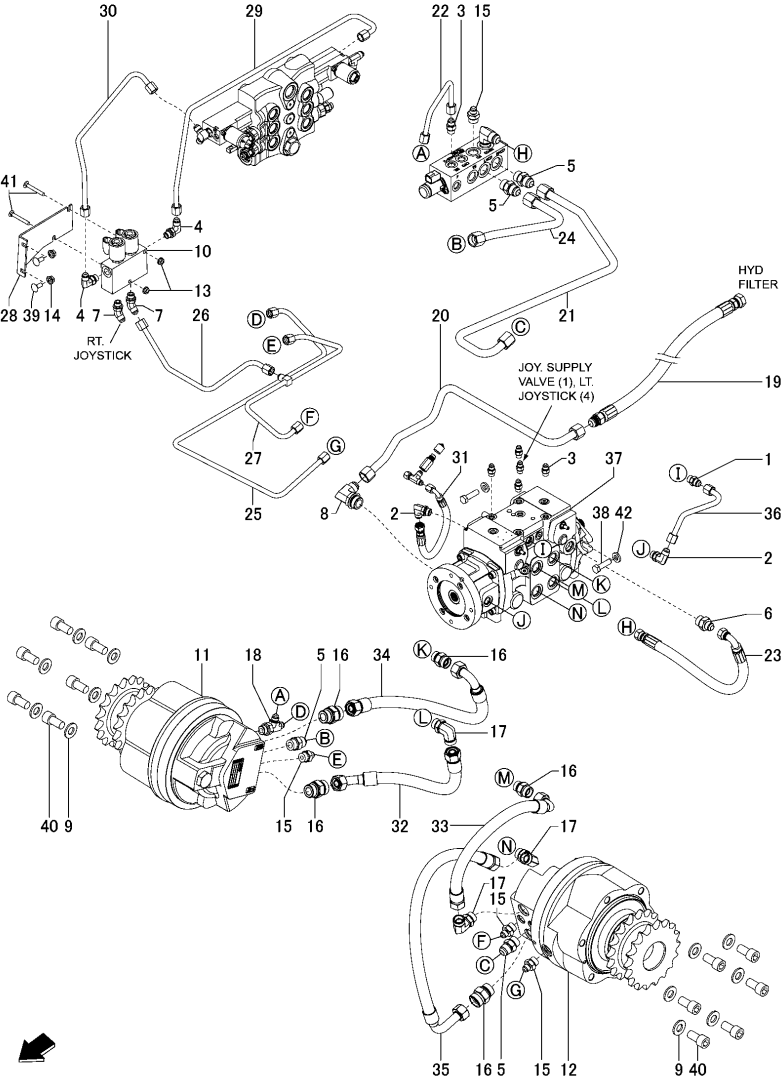
Fig.46. HYDROSTATICS WITH DRIVE MOTORS(2-SPEED JOYSTICK CONTROLS)
