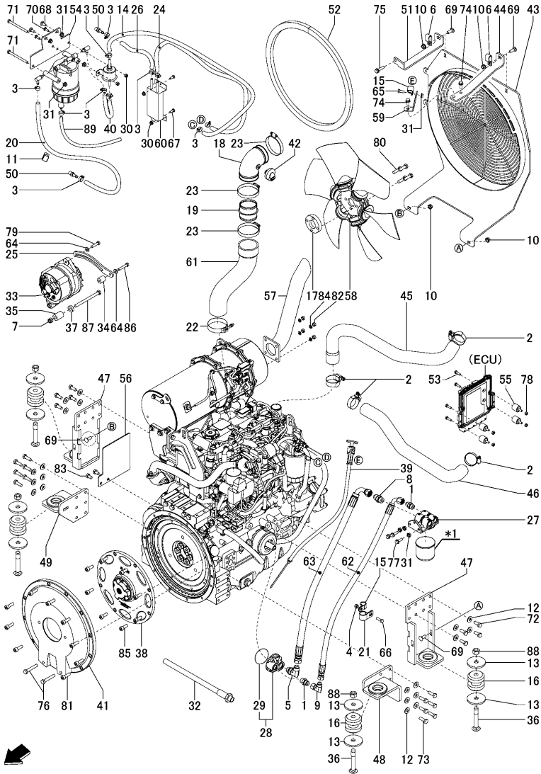
OCK50-M00570 ENGINE Fig.26. ENGINE
